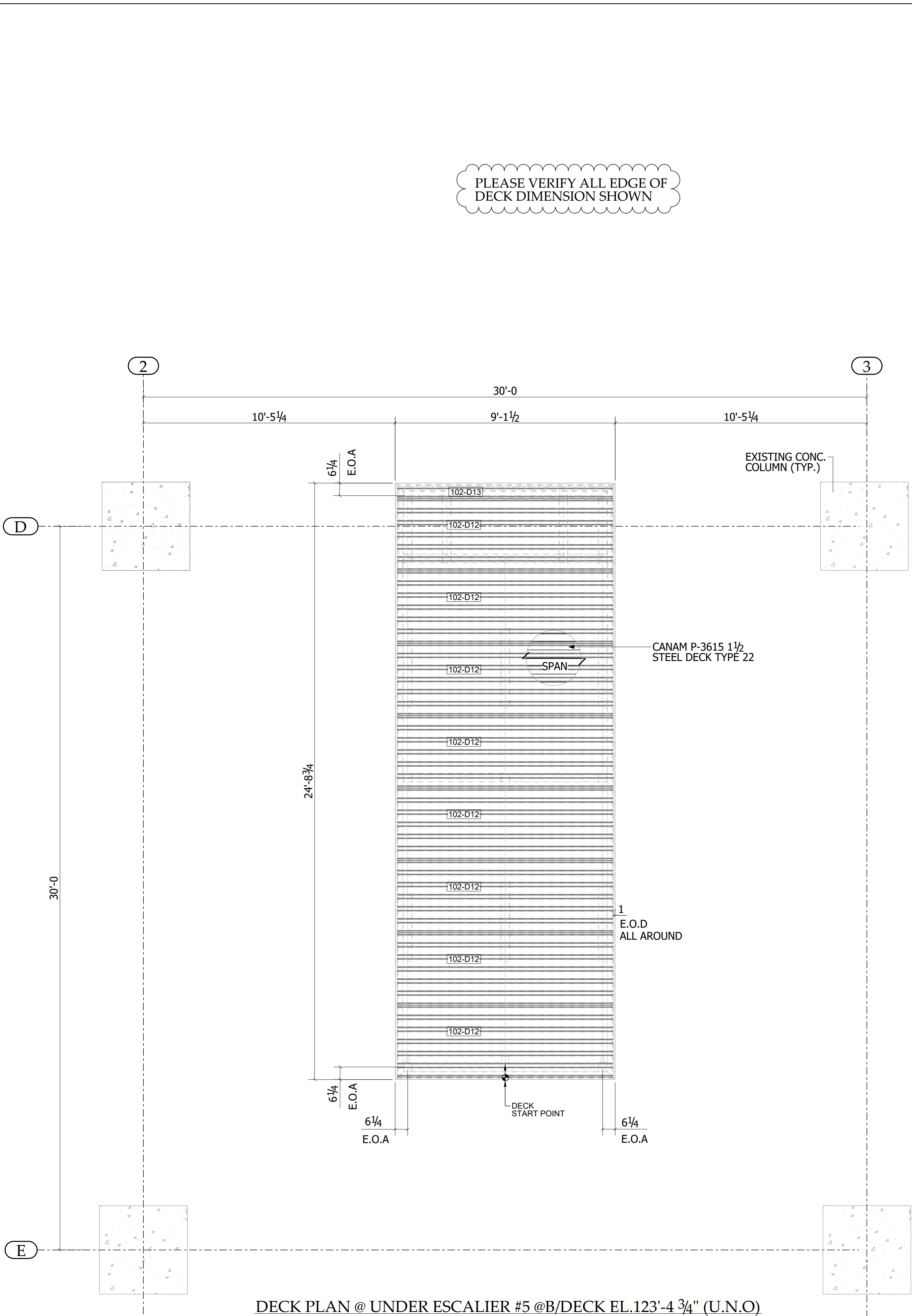
DECK PLAN @ UNDER ESCALIER #5 @B/DECK EL.123'-4 3/4" (U.N.O)
