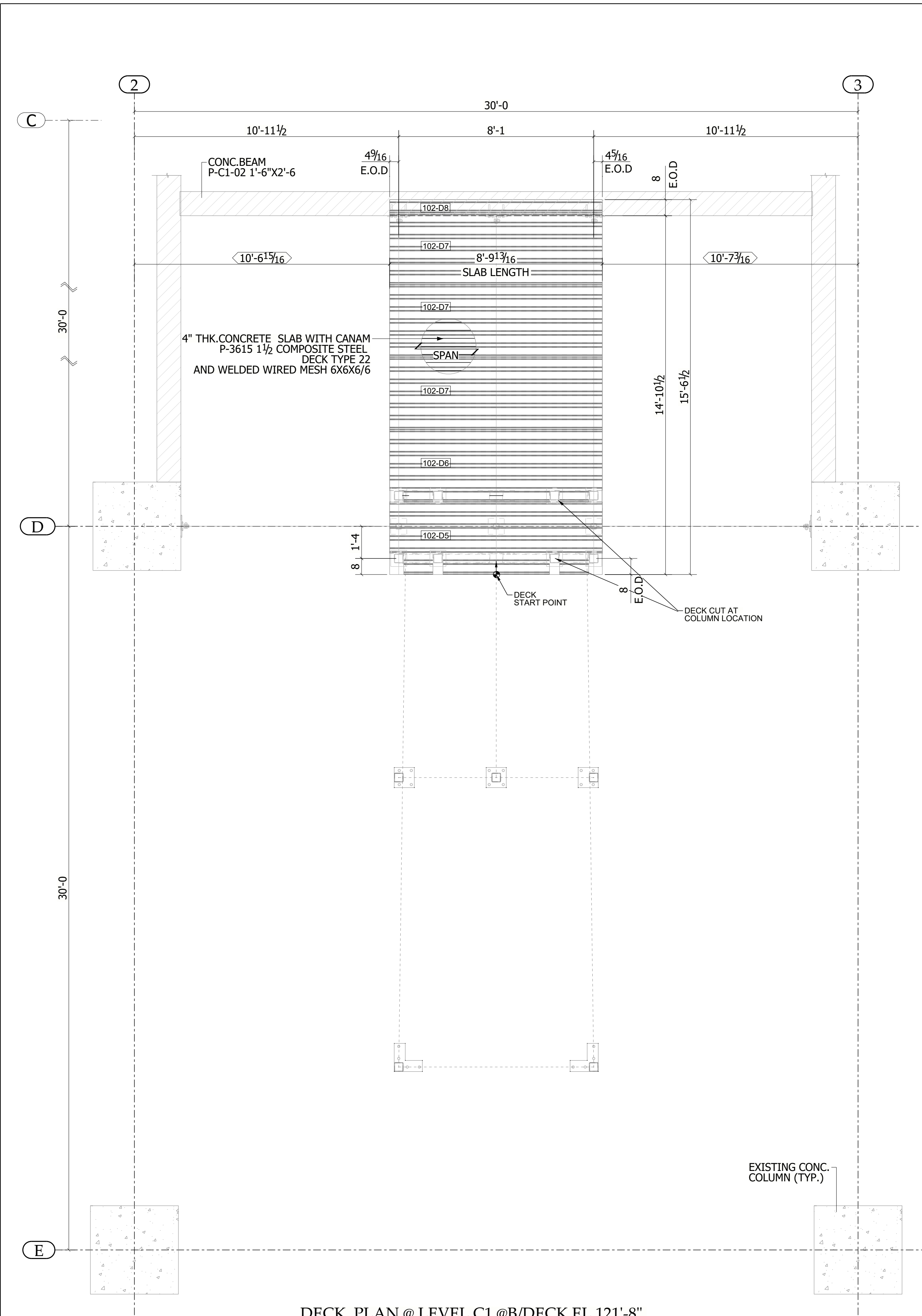
DECK PLAN @ LEVEL C1 @B/DECK EL.121'-8"
